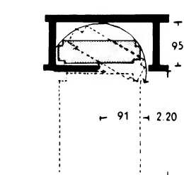
20 Hinged/swinging folding beds
